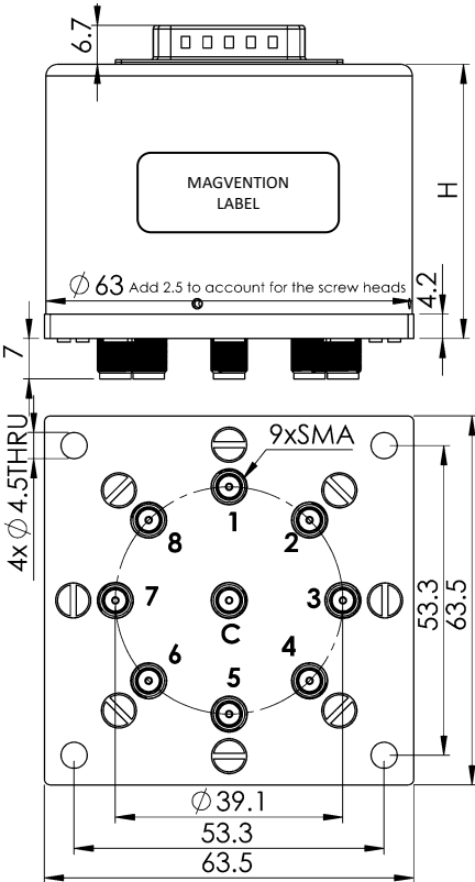
Mechanical drawings (unit: mm, tolerance +/-0.5mm).
